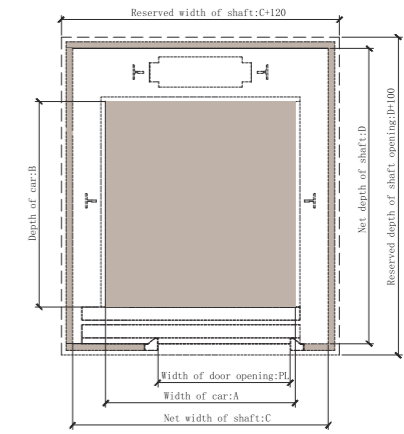
Layout plan of hoistway-side door
