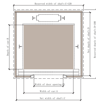
Layout plan of the hoistway-central opening
