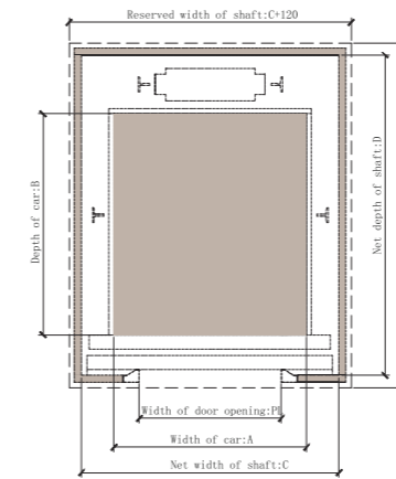
Layout plan of hoistway-central opening with bifolding door
