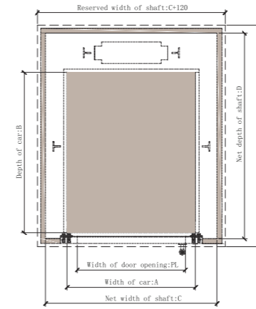
Layout plan of hoistway-hand pulled door
