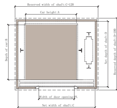
Layout plan of the hoistway-central opening
