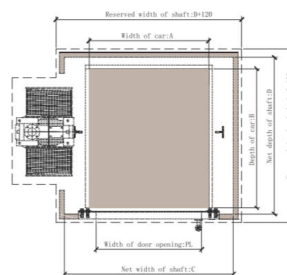
Floor plan of down-mounted shaft
