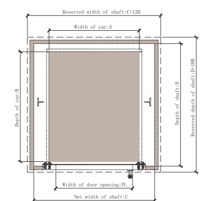
Plane layout of top-mounted shaft
